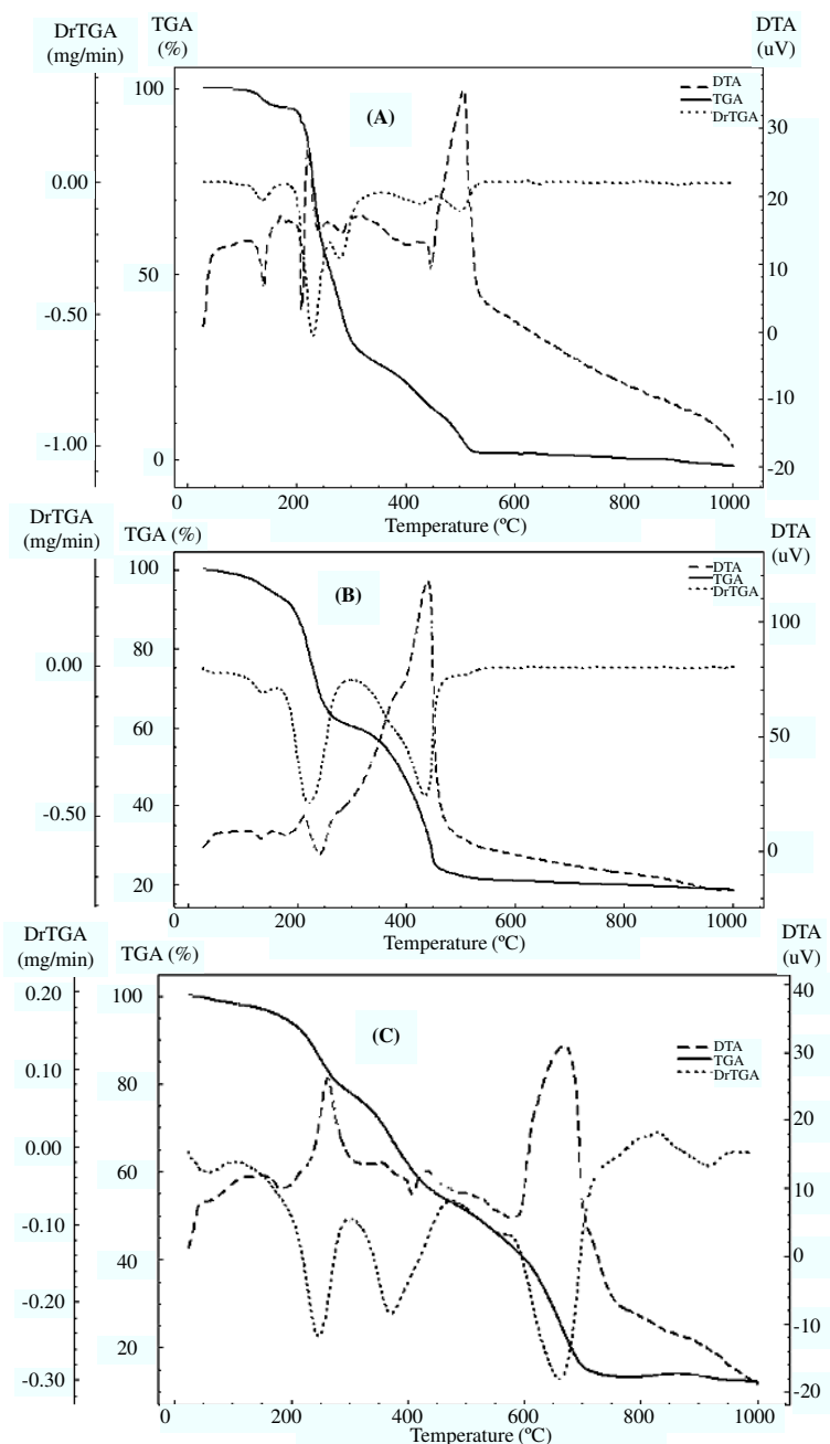
Fig. 1. Thermal analyses (TG, DTG and DTA) of \text{H}_2\text{L} and its complexes. Where (A) \text{H}_2\text{L} ligand, (B) \text{Cr(III)} and (C) \text{Zn(II)} complexes
